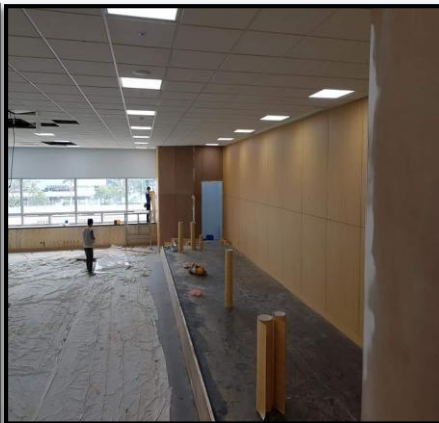
HYUNDAI KEFICO FACTORY CONFERENCE ROOM Interior Works – Hải Dương
